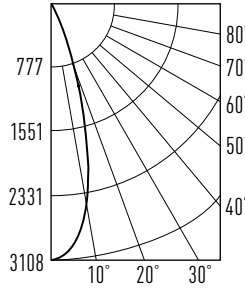
30° Flood (-30)
