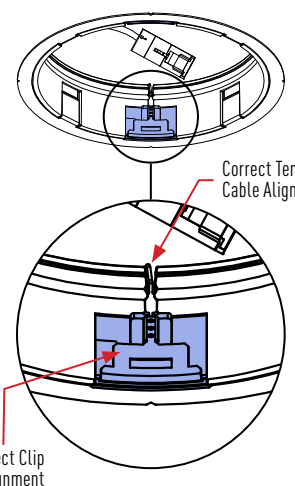
Detail View
