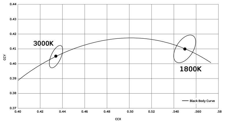
CCT Range in Warm Dimming Mode
