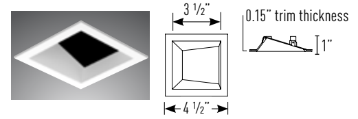
MXTG2-STRA300 (1" Regress)
