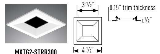
MXTG2-STRR300 (1/2" Regress)
