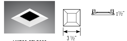
MXTG2-STLR300 (1/2" Regress Trimless)
