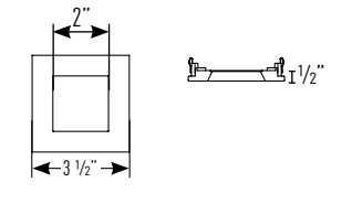
MXTG2-STLR306 (1/2" Regress Trimless)
