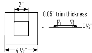
MXTG2-SFRR306 (1/2" Flat Mount)
