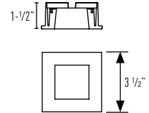
MXTG2-STLD306 (1-1/2" Regress Trimless)
